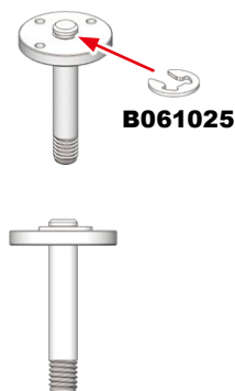
ASSEMBLY VIEW
